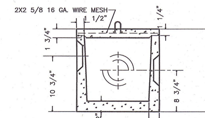
STANDARD D-BOX
