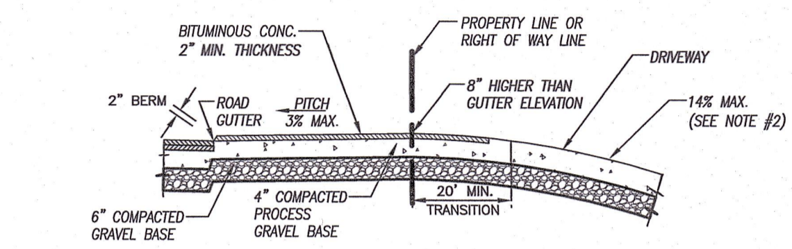
LAND BELOW ROAD (SECTION)
