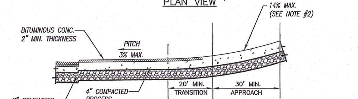
LAND ABOVE ROAD (SECTION)
