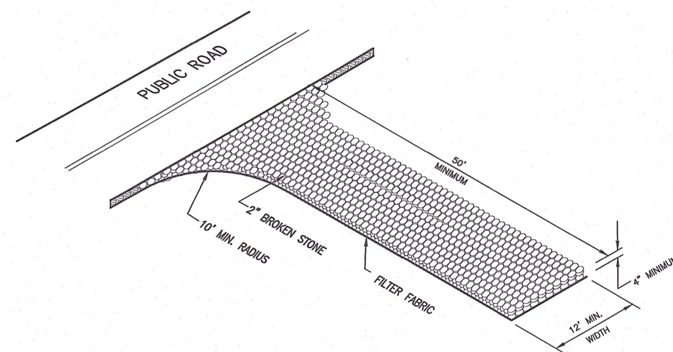
ANTI-TRACKING PAD
