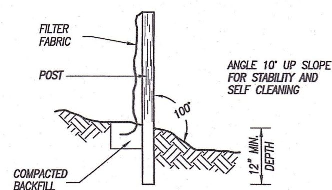
SILT FENCE
